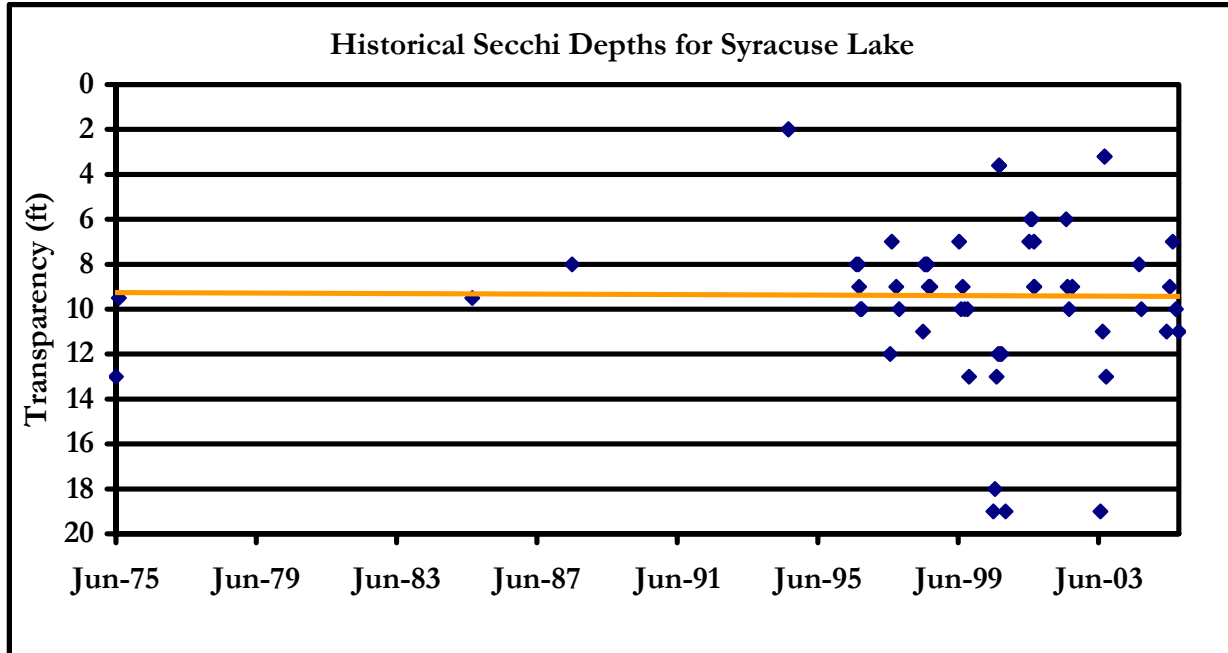
Figure 21. Secchi disk transparencies measured in Syracuse Lake, 1975 to 2005.
