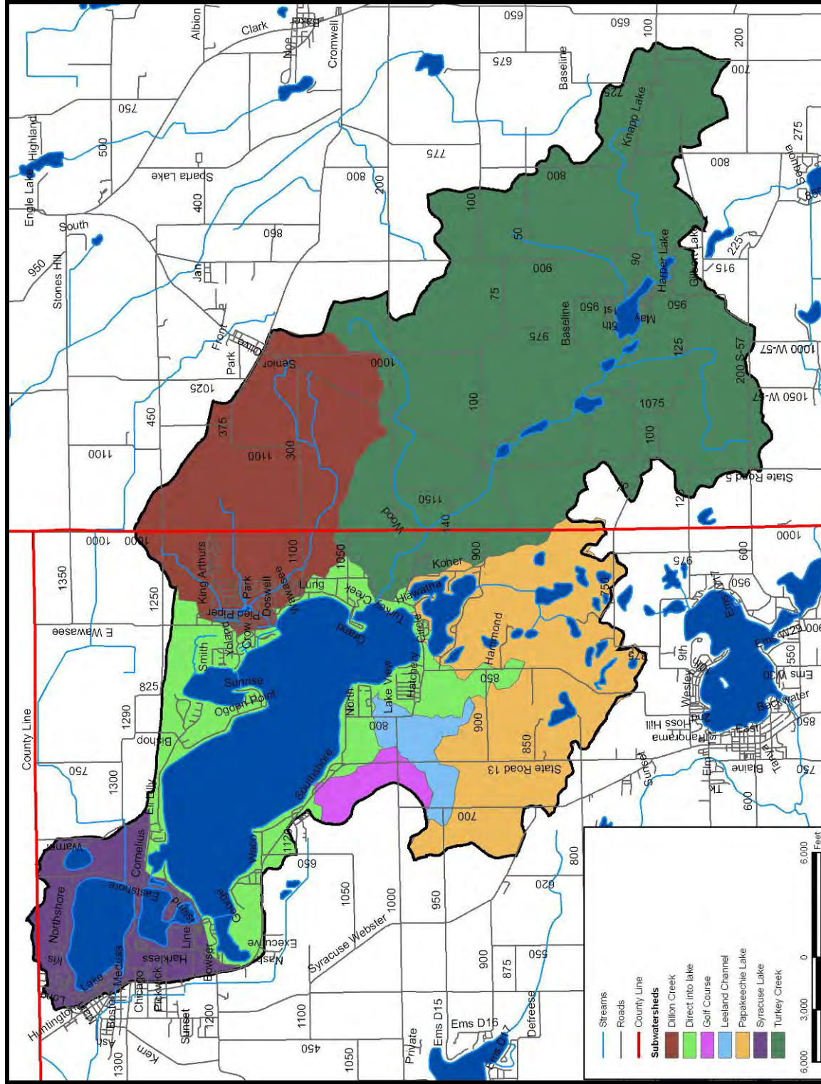
Figure 3. Lake Wawasee subwatersheds.
