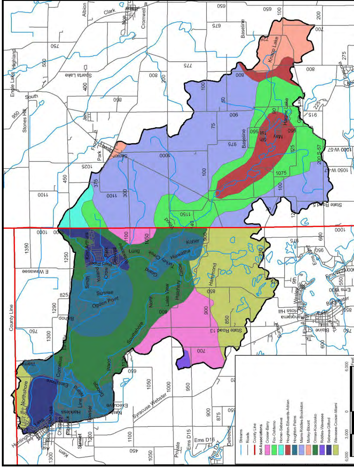
Figure 7. Soil associations present in the Wawasee Area Watershed.
