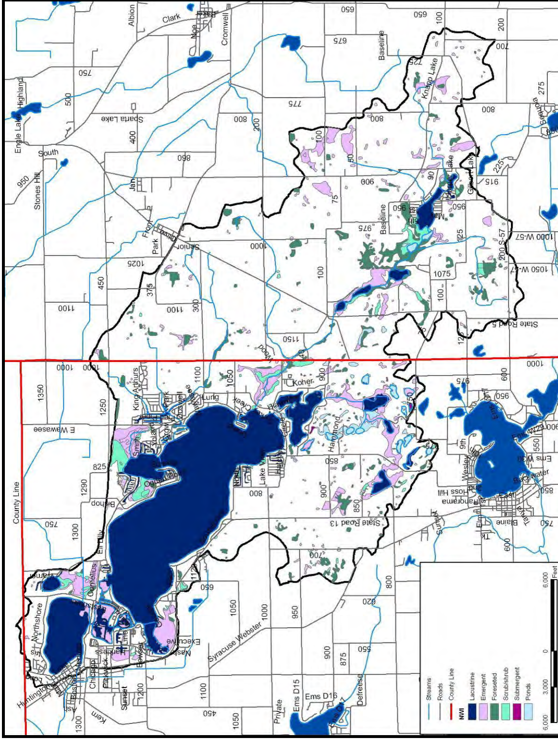
Figure 11. Wetland locations within the Wawasee Area Watershed.
