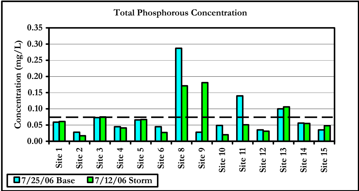
Figure I8. Total phosphorus concentrations measured during base flow and storm flow sampling of Wawasee Area Watershed streams.
