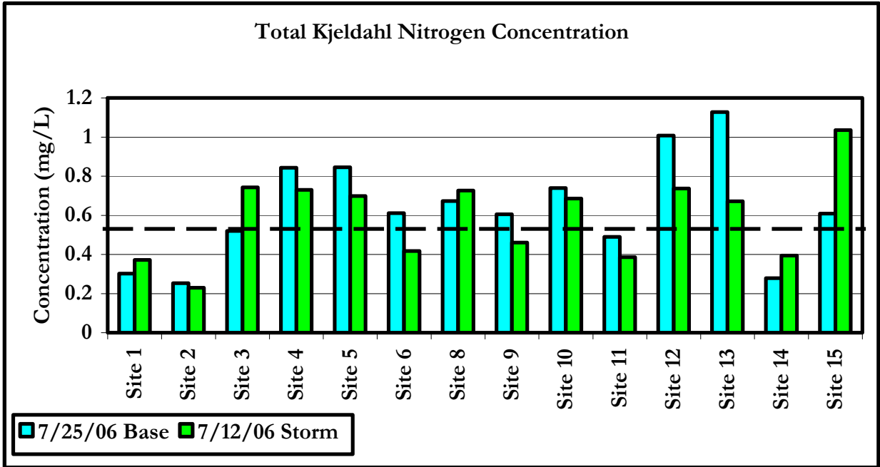
Figure I7. Total Kjeldahl nitrogen concentrations measured during base flow and storm flow sampling of Wawasee Area Watershed streams.
