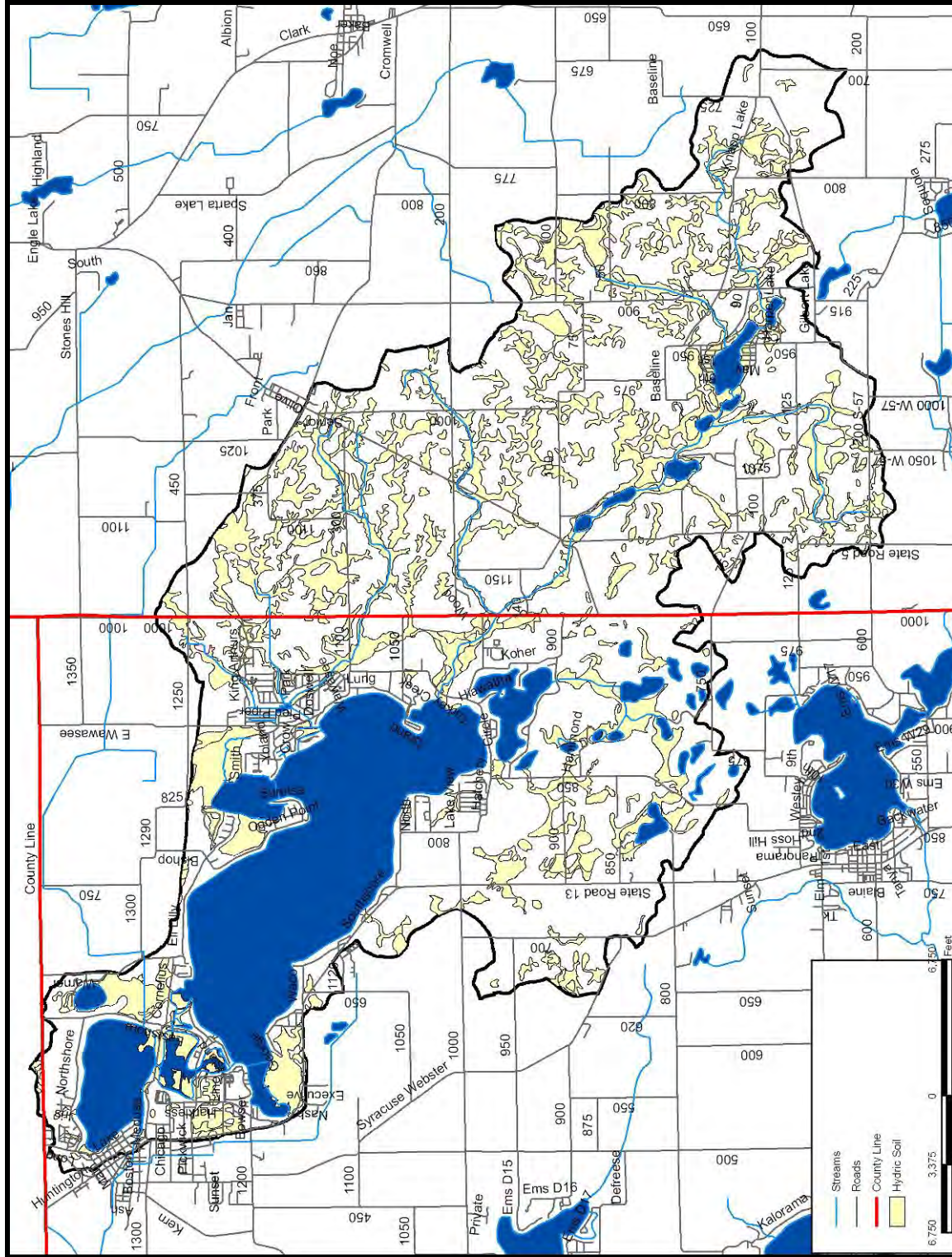
Figure 12. Hydric soils in the Wawasee Area Watershed.
