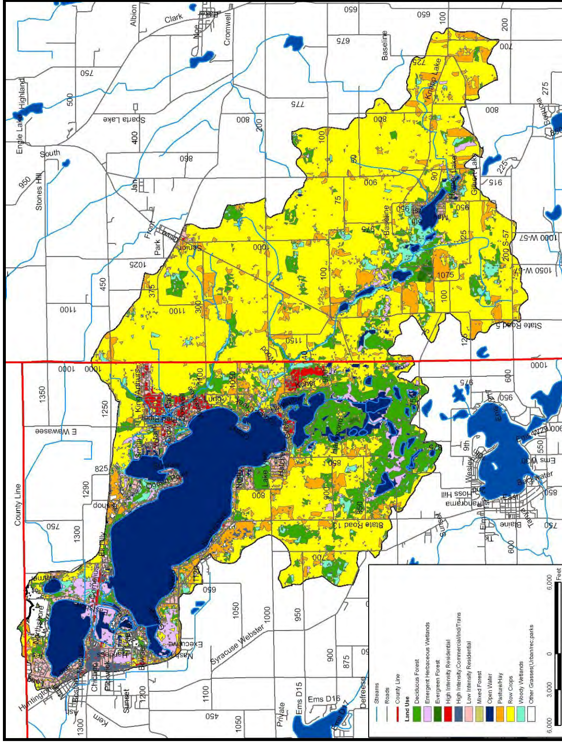
Figure 17. Land use in the Wawasee Area Watershed.
