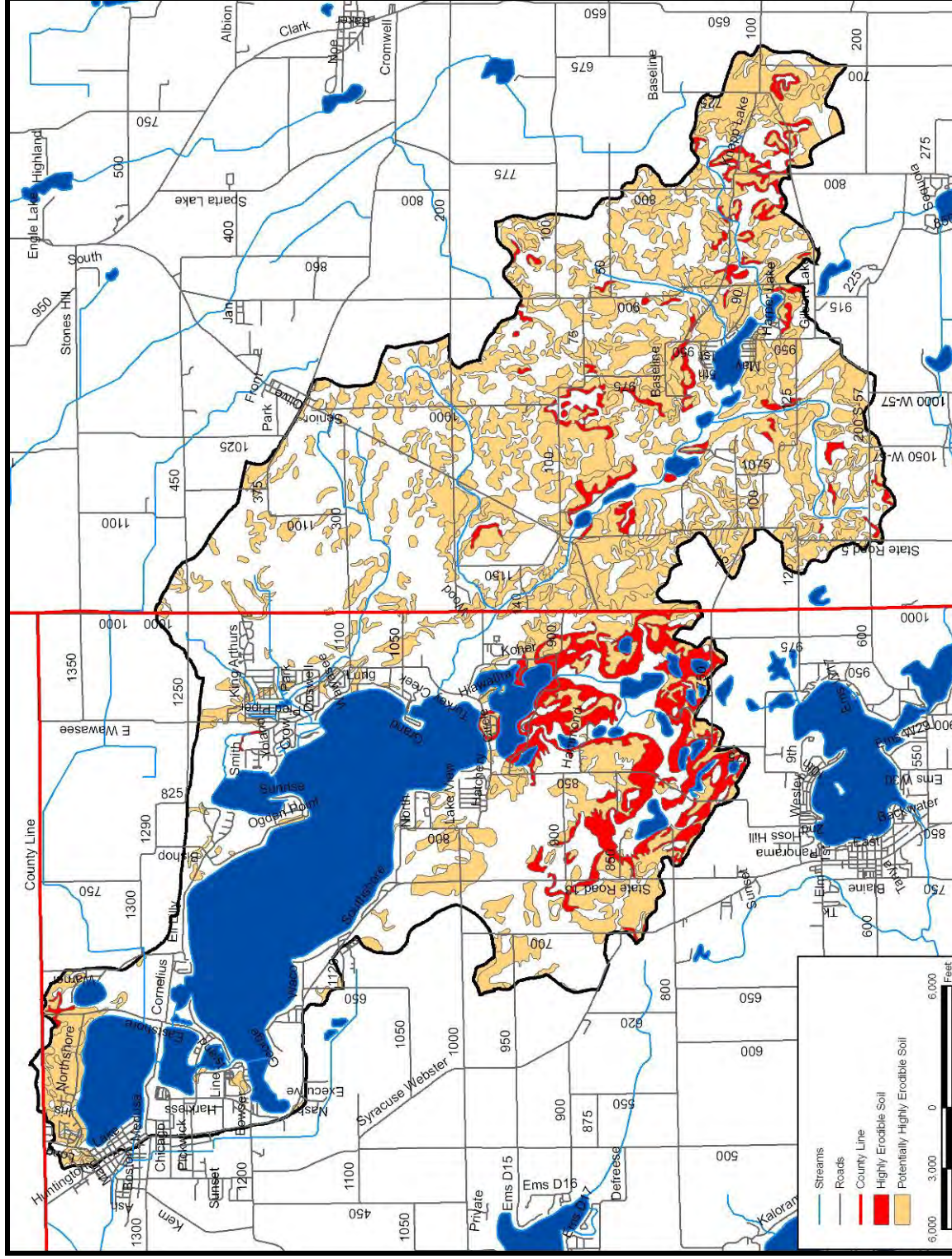
Figure 8. Highly erodible and potentially highly erodible soils in the Wawasee Area Watershed.
