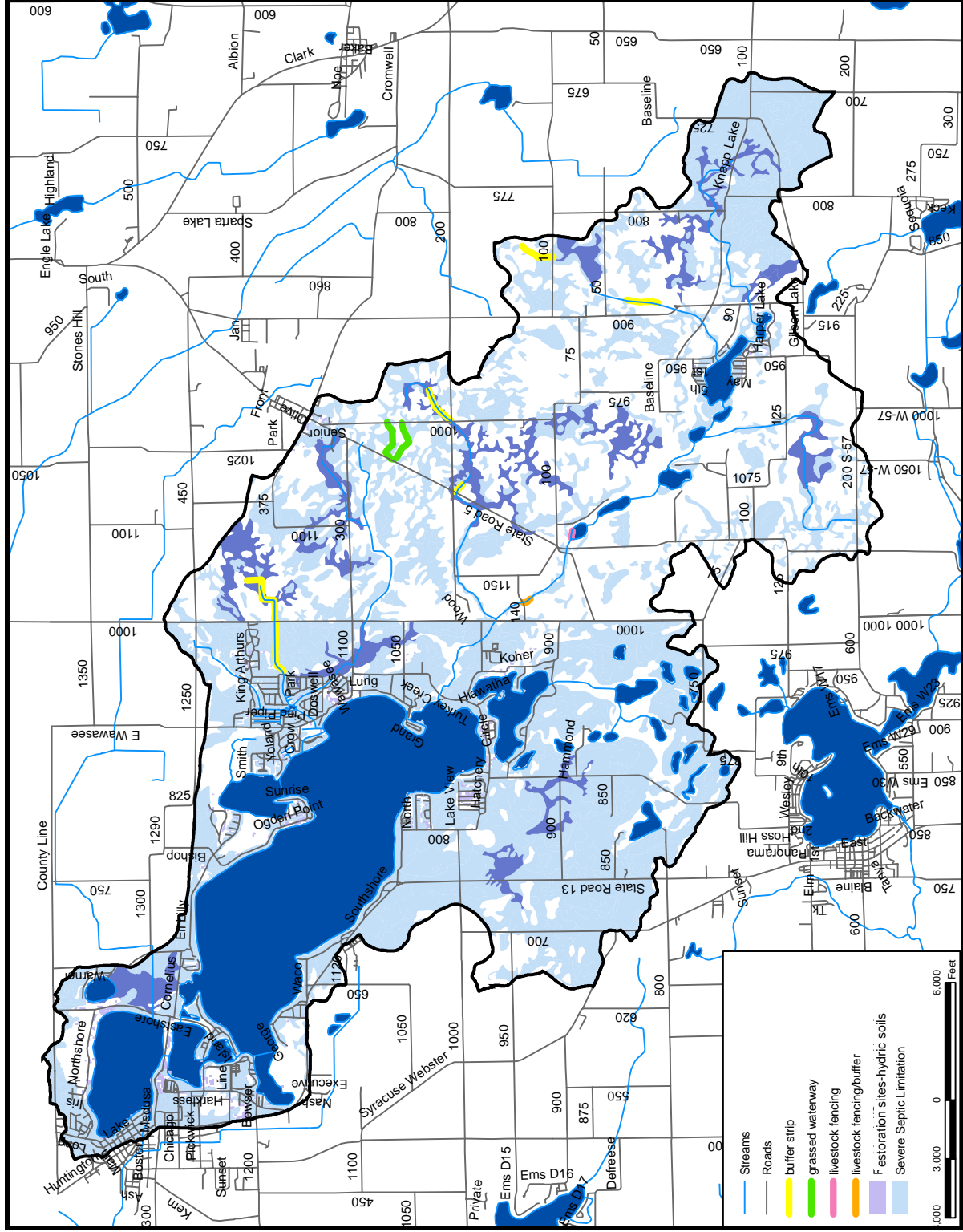
Figure 32. Critical areas targeted for nutrient loading and pathogen concentration reduction in the Wawasee Area Watershed.
